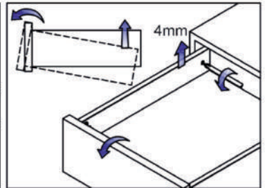
Front slope angle adjustment
