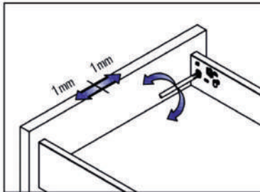
Left&right adjustment
