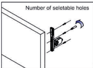
121 Front assembly
