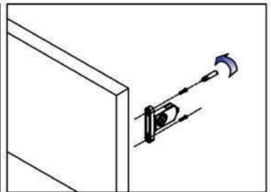
89 Front assembly
