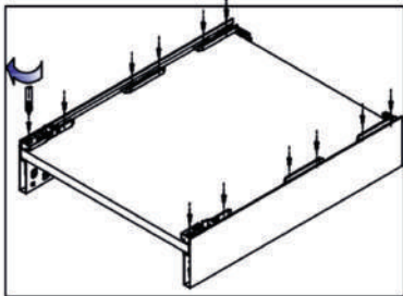
Bottom assembly
