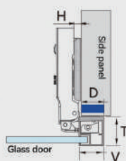
Half overlay
