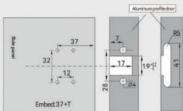
Full overlay
