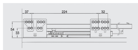
Location of side plate mounting ( Gallery)
