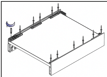
Bottom assembly
