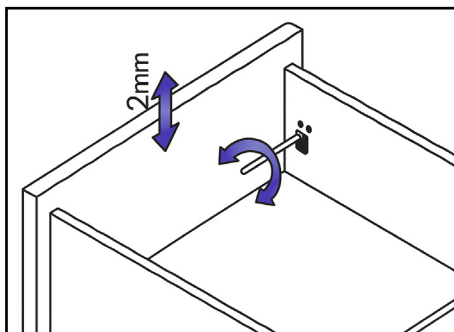
Up & down adjustment
