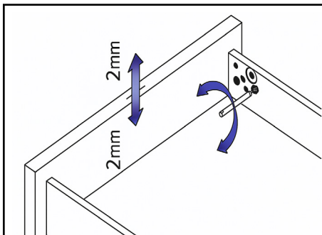
Up & down assembly
