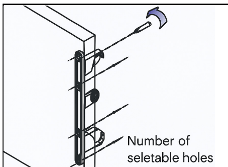
Front assembly
