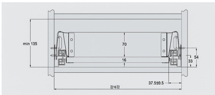
Location of side plate mounting ( In box)
