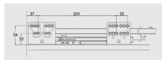
Location of side plate mounting (Drawer)
