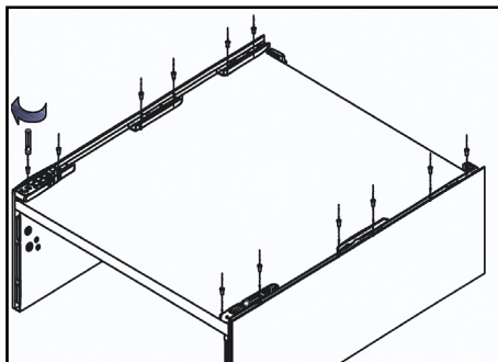
Bottom assembly
