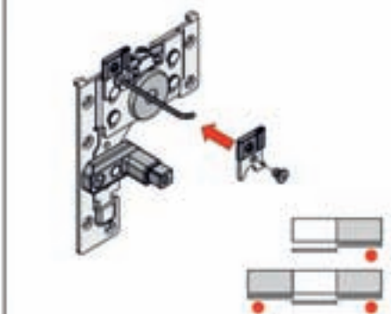
Install upper/lower rollers on the doors
