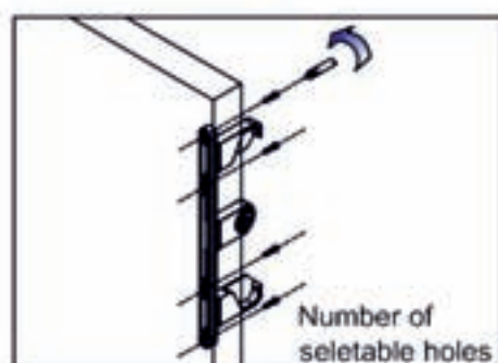
Front assembly
