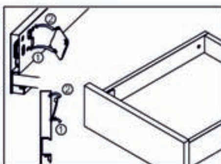
89 Front assembly
