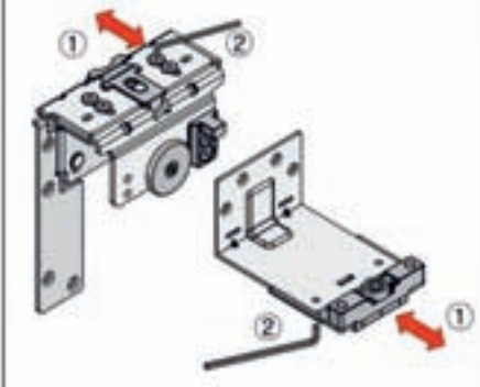
Unfasten vertical adjustment bolt (0mm)
