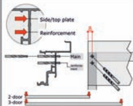
Drill on interior side of top plate
