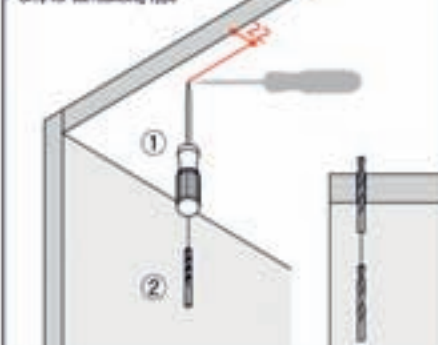
Drill on the bottom plate & install lower rail
