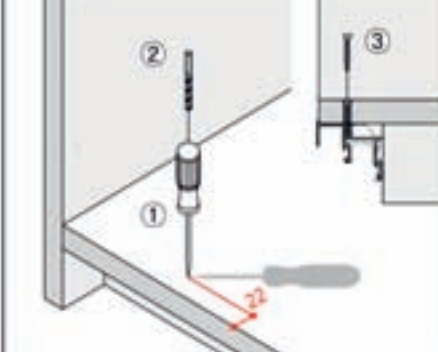
Install inner door stopper for 3-door-type
