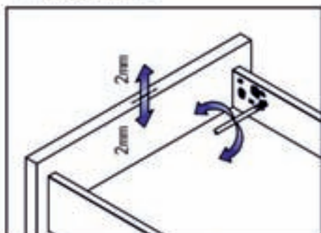
Up&down adjustment
