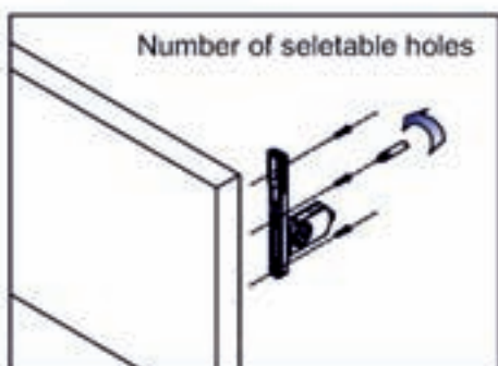
121 Front assembly
