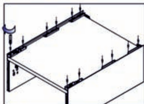
Bottom assembly
