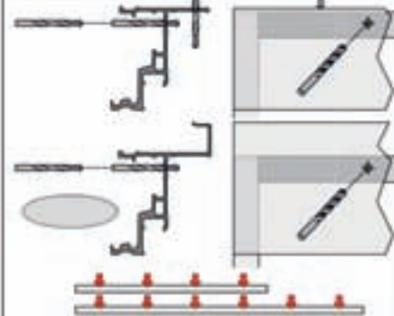
Fix rail position with nails
