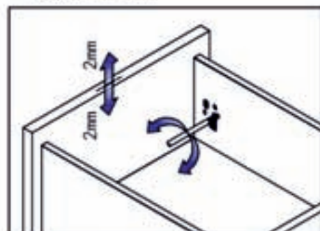
Up&down adjustment
