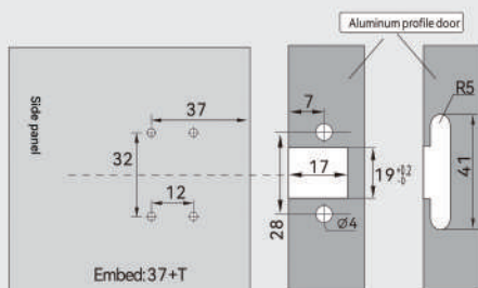
Full overlay
