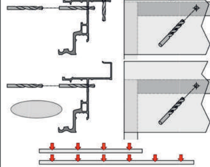
Fix rail position with nails
