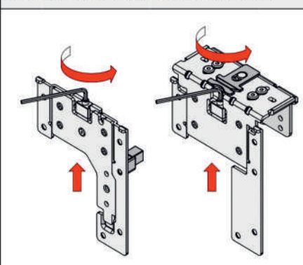
Unfasten vertical adjustment bolt (0mm)
