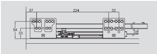
Location of side plate mounting ( In box)
