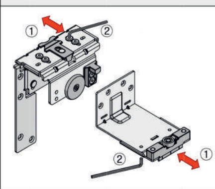
Adjust depth of outer roller (initial D=22)
