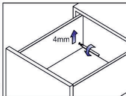
Front slope angle adjustment
