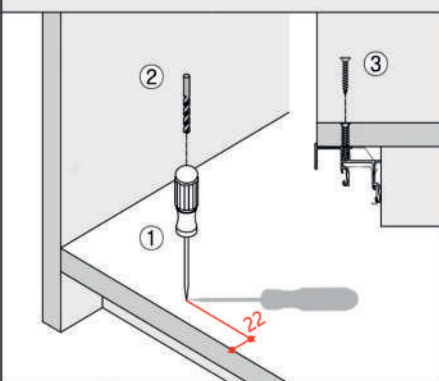
Drill on the bottom plate & install lower rail
