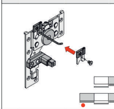
Install handle guard & inner upper roller
