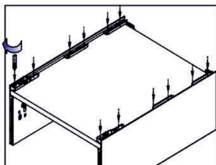
Bottom assembly
