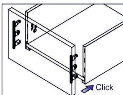
Back assembly
