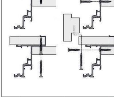
Install handle guard & inner upper roller
