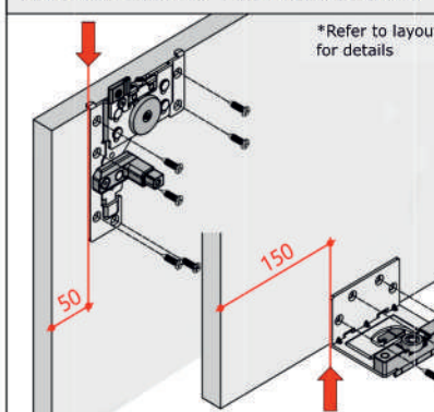
Install upper/lower rollers on the doors
