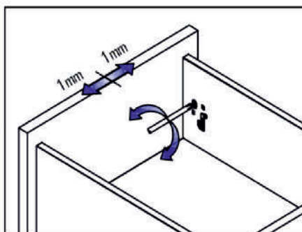
Left&right adjustment
