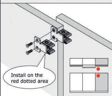
Install inner door stopper for 3-door-type
