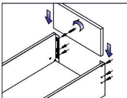
Back assembly
